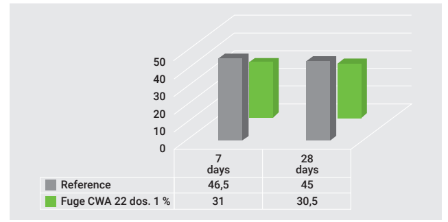
Water penetration under pressure (mm)
