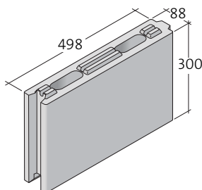
Leca® EasyLex 88 VS harkko *)
